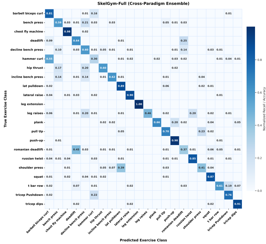
Fig. 5: Normalized confusion matrix of the proposed SkelGym-Full cross-paradigm ensemble evaluated on held-out test windows ( N = 2,743 ).
