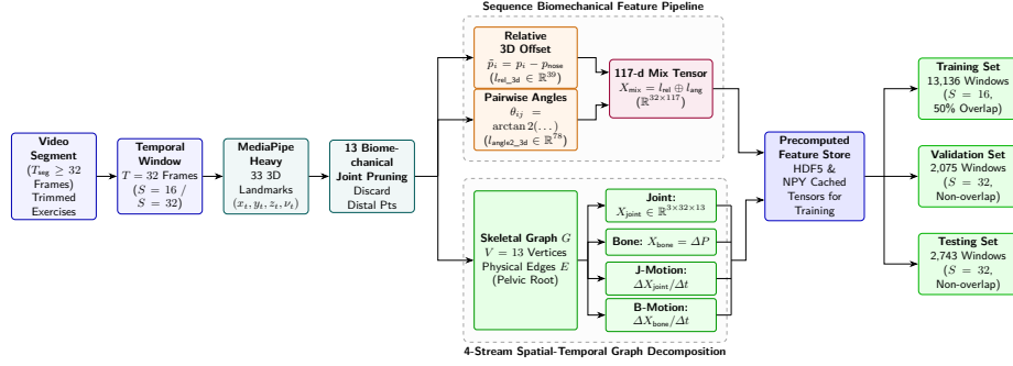
Fig. 4: The proposed Biomechanical Feature Extraction and Kinematic Tensor Decomposition pipeline: illustrating the two-branch extraction of the 117-d sequence mix and the 4-stream spatial-temporal graph tensors.
