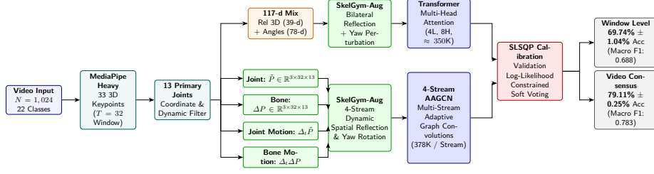
Fig. 1: The proposed SkelGym architecture: an end-to-end cross-paradigm framework coupling self-attention sequence modeling with multi-stream adaptive graph convolutional networks via validation-calibrated weighted soft voting.
