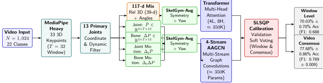
Figure 1: The proposed SkelGym architecture: an end-to-end cross-paradigm framework coupling self-attention sequence modeling with multi-stream adaptive graph convolutional networks via validation-calibrated weighted soft voting.
