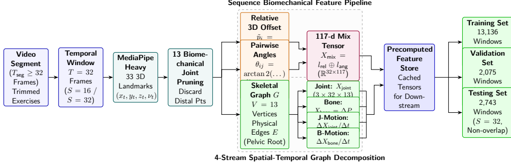
Figure 4: The proposed Biomechanical Feature Extraction and Kinematic Tensor Decomposition pipeline: illustrating the two-branch extraction of the 117-d sequence mix and the 4-stream spatial-temporal graph tensors.
