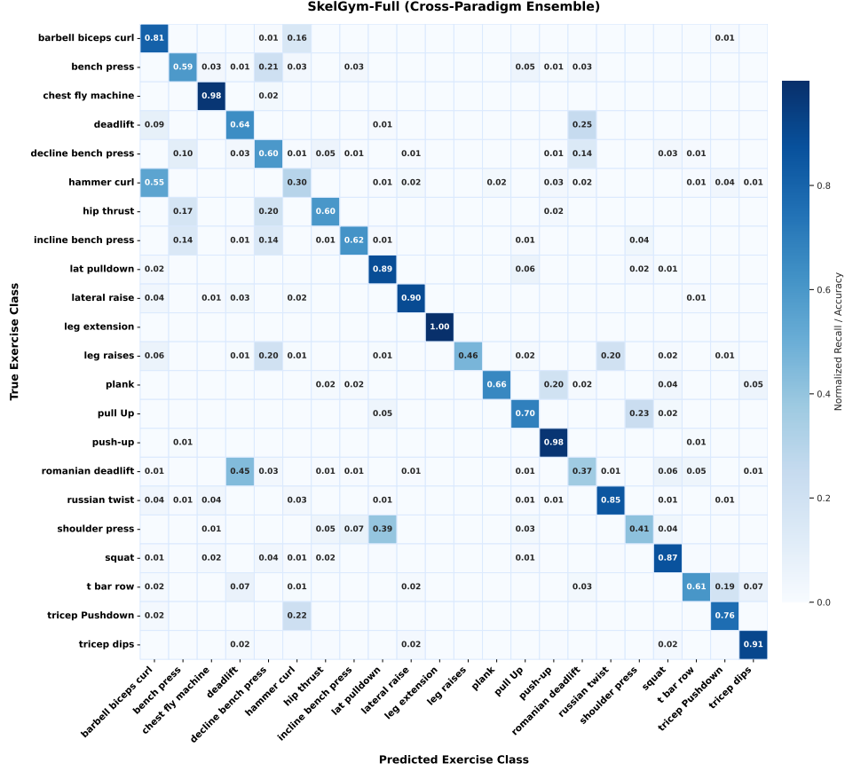
Figure 5: Normalized confusion matrix of the proposed SkelGym-Full cross-paradigm ensemble evaluated on held-out test windows ( N = 2,743 ).
