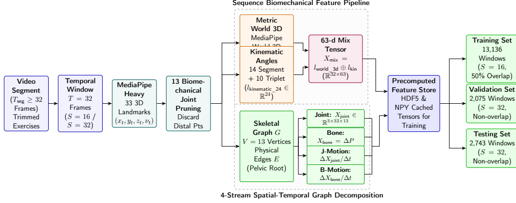
Figure 4: The proposed Biomechanical Feature Extraction and Kinematic Tensor Decomposition pipeline: illustrating the two-branch extraction of the 63-d sequence mix and the 4-stream spatial-temporal graph tensors.
