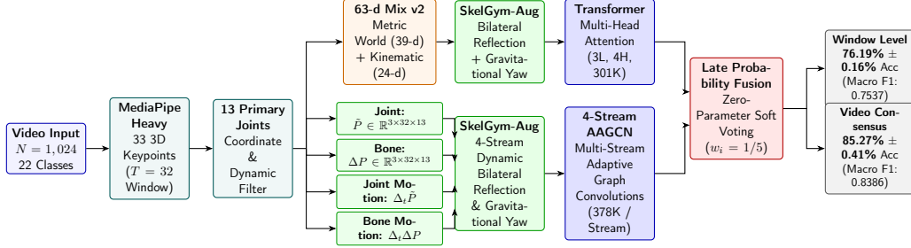
Figure 1: The proposed SkelGym architecture: an end-to-end cross-paradigm framework coupling self-attention sequence modeling with multi-stream adaptive graph convolutional networks via zero-parameter uniform average soft voting.
