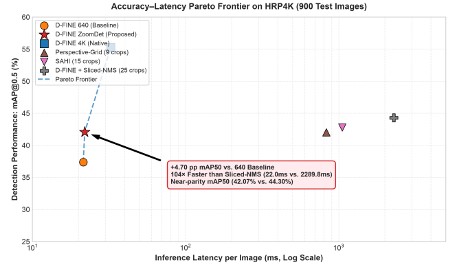
(b) Fig. 2: Accuracy-Latency Pareto Frontier (mAP@0.5).
