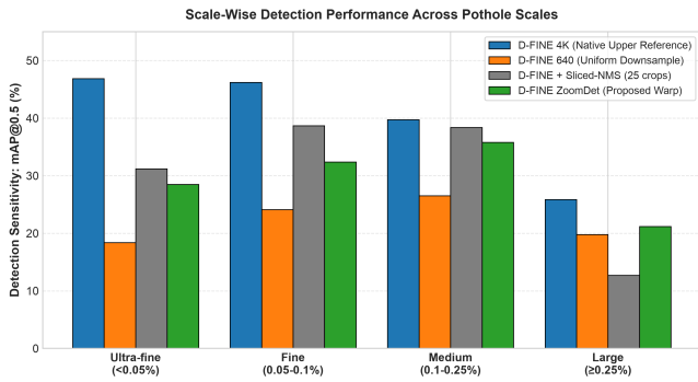
(c) Fig. 3: Scale-Wise Detection Performance (mAP@0.5).
