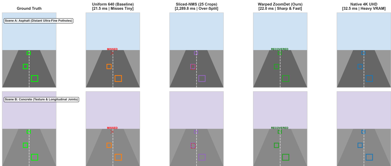
Figure 4: Fig. 7: Qualitative Detection Comparison. Visualizing detection results across representative test scenes: Ground Truth (Green), Uniform 640 Baseline (Missed far targets), Sliced-NMS (Over-split boundary boxes), Warped ZoomDet (Accurately recovered in single pass at 22.0 ms), and Native 4K UHD (Upper reference).
