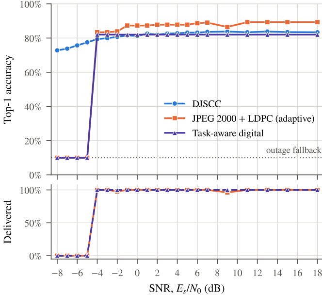
Fig. 1. Validation accuracy (top) and fraction of packets delivered (bottom) at r = 1/6 . DJSCC is scored by its own task head, and JPEG 2000 by the ResNet-18 fine-tuned on JPEG 2000 artifacts. The dotted line is the 10% outage rule. The digital systems re-select their operating point at every SNR on validation data; DJSCC is trained once at 7 dB. Lines join measured points only.
