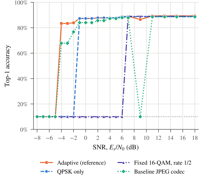
Fig. 5. Adaptive JPEG 2000 + LDPC at r = 1/6 against restricted versions: QPSK only (rate and resolution still adapted), one fixed operating point at all SNRs, and baseline JPEG in place of JPEG 2000. All scored by the fine-tuned ResNet-18.
