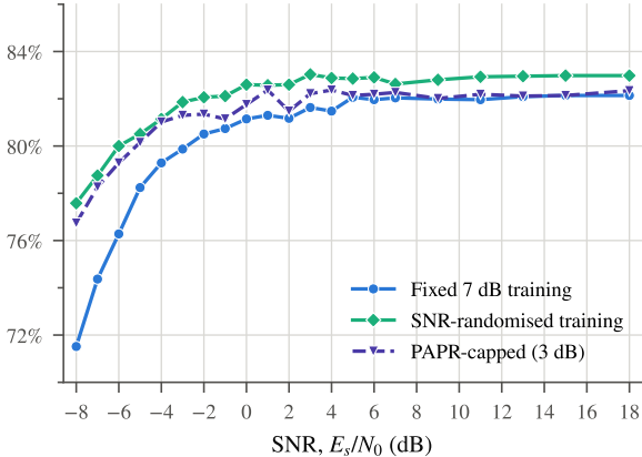
Top-1 accuracy
