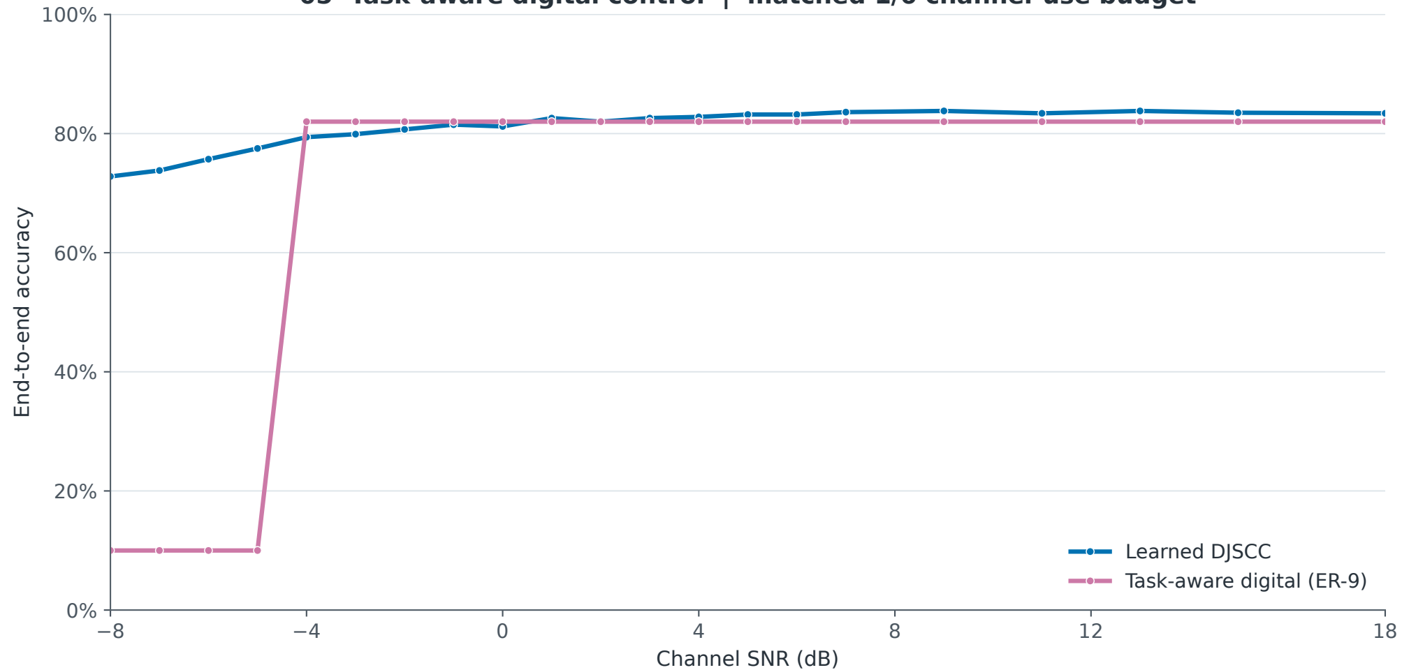
05 Task-aware digital control | matched 1/6 channel-use budget
