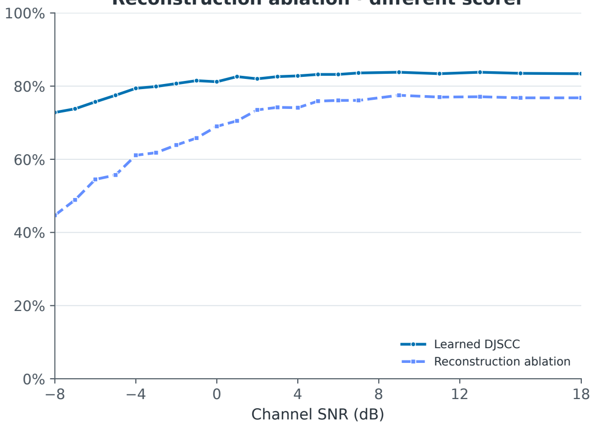
Reconstruction ablation · different scorer
