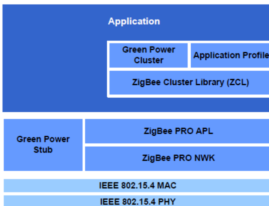
Figure 2. ZigBee Green Power Software Stack
