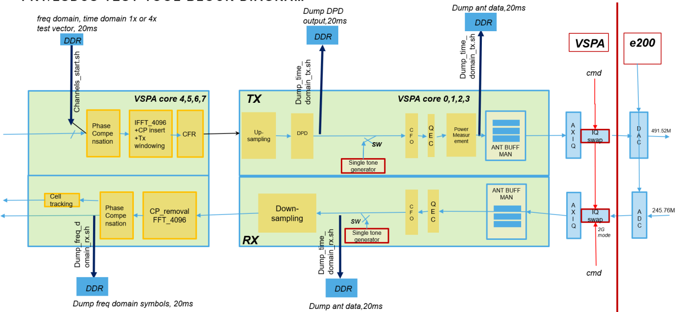
FR1/LSDCS TEST TOOL BLOCK DIAGRAM
