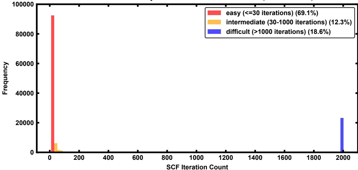
SCF Iteration Summary for QM9 Doublet Anion Molecules (UHF/6-31++G**)
