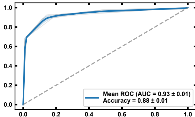
Gradient Boosting
