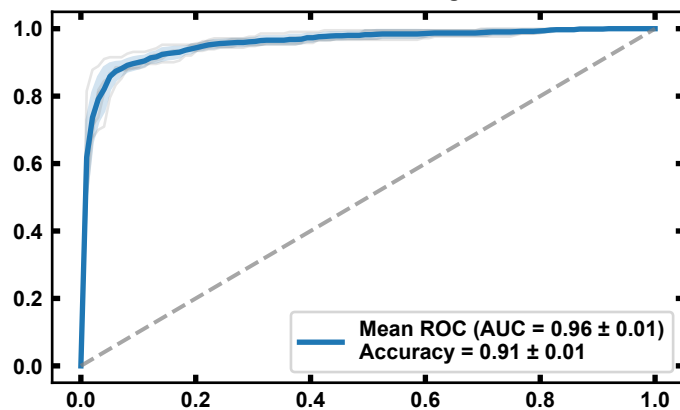
Gradient Boosting
