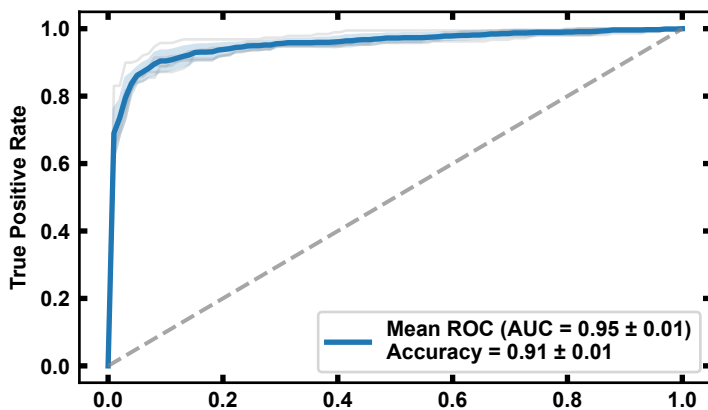
Random Forest
