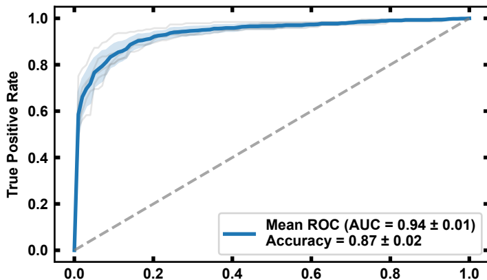
Random Forest
