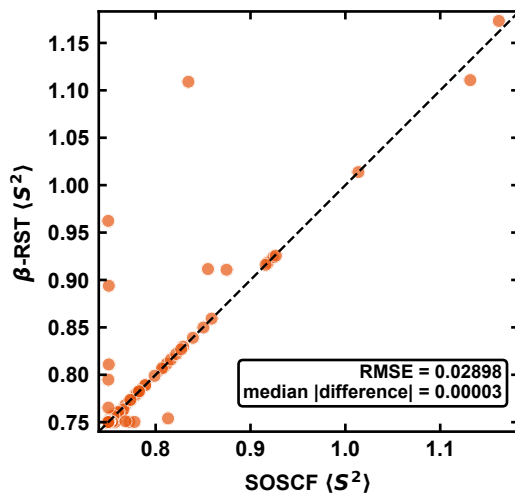
\langle S^2 \rangle comparison
