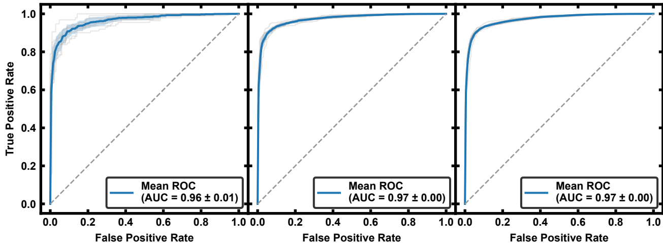
iSmall-train
