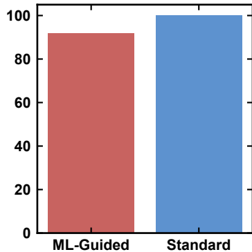
Convergence Rate (%)
