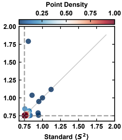
ML-Guided ( S^2 )
