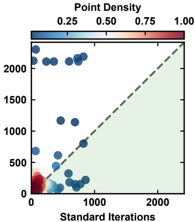
ML-Guided Iterations
