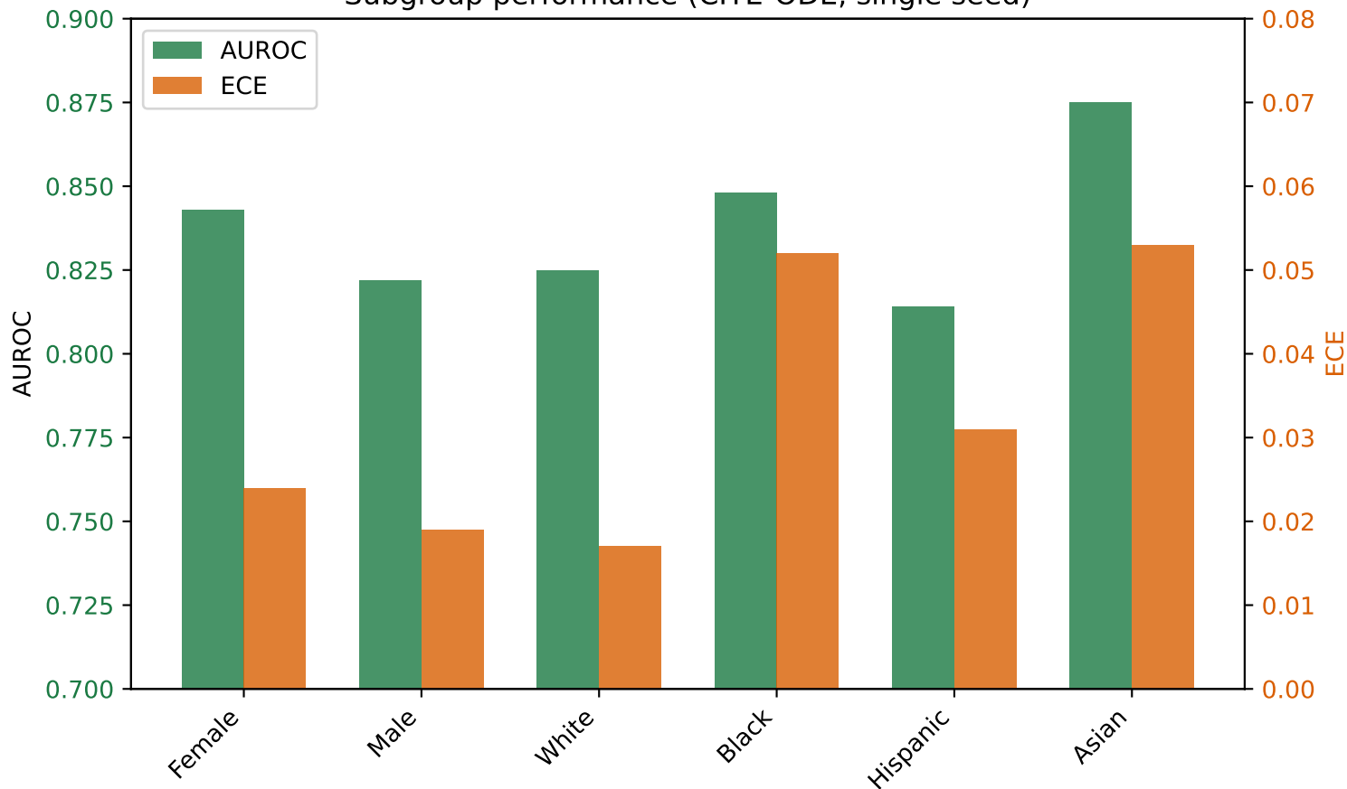
Subgroup performance (CITE-ODE, single seed)
