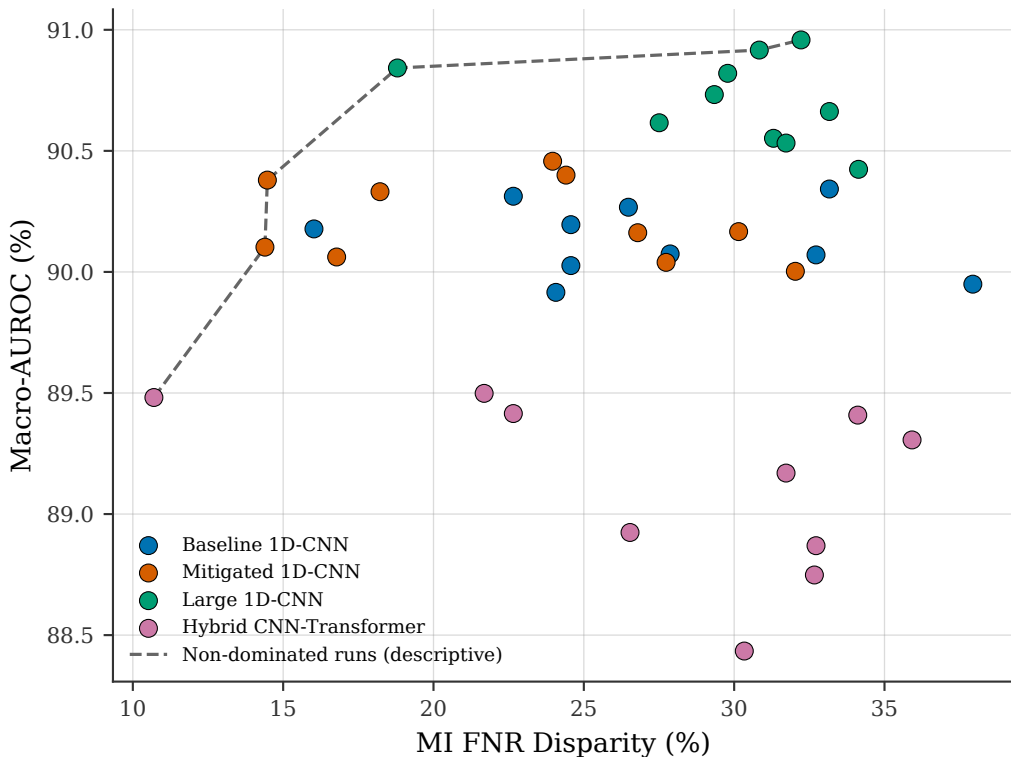
Performance vs. Fairness — Empirical Association Across Runs (descriptive only; not a model-selection criterion)
