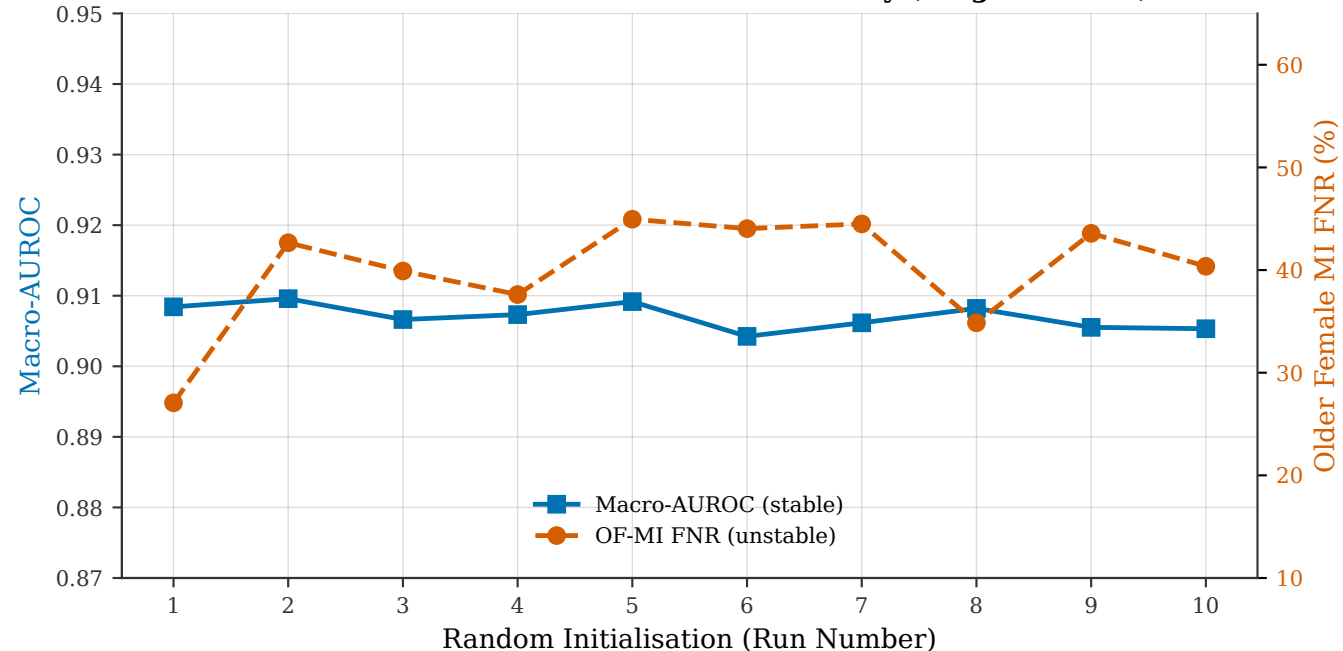
Predictive Performance vs. Fairness Stability (Large 1D-CNN)
