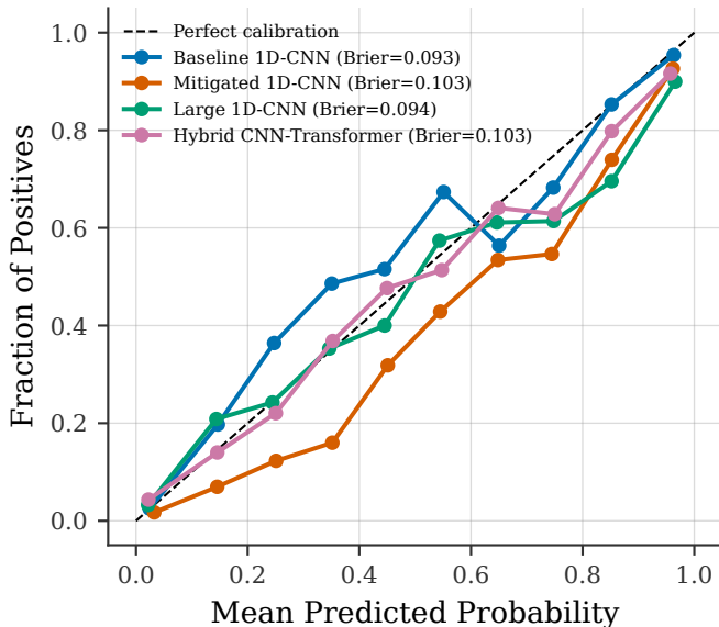
Reliability Diagram — MI
