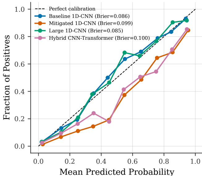
Reliability Diagram — STTC
