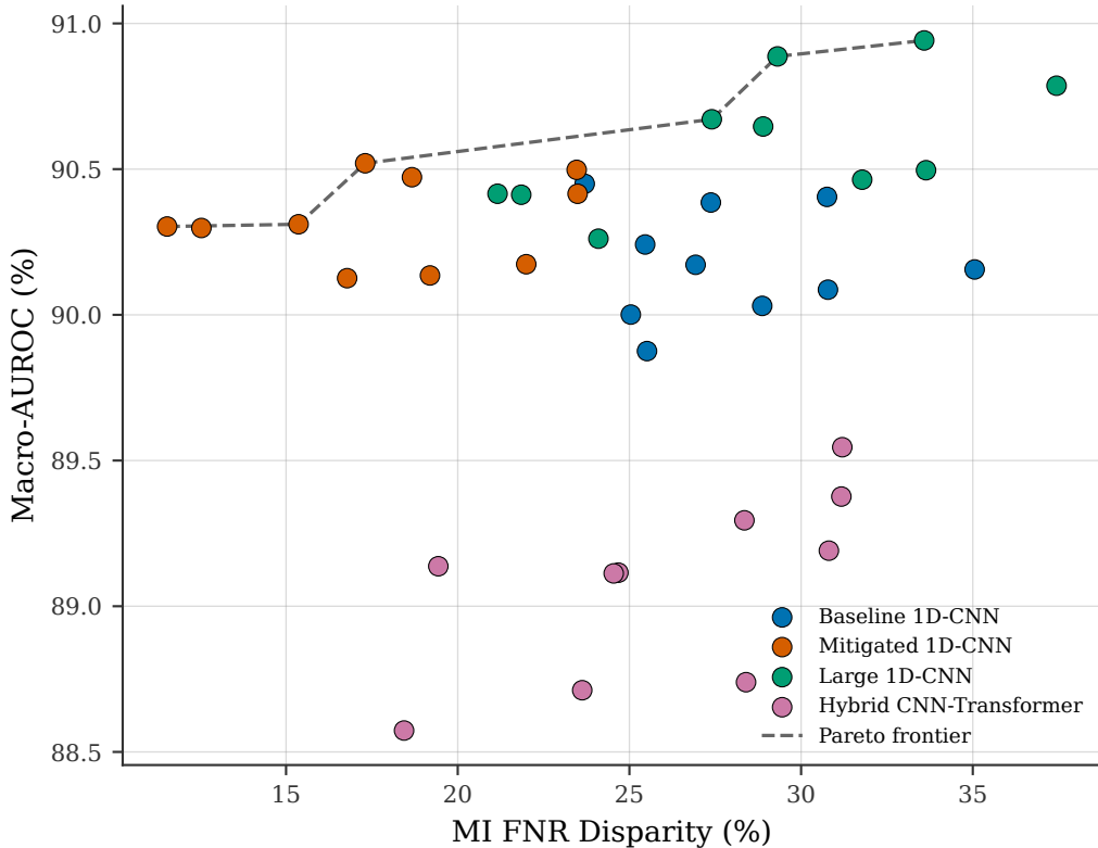
Performance vs. Fairness Trade-off Across All Runs
