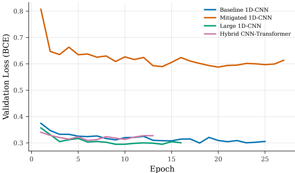
Validation Loss Convergence — All Models (Seed 42)
