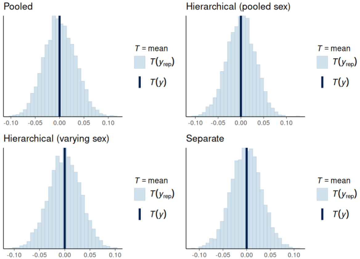
Posterior predictive checks for the mean across all four models. The dark line is the observed mean of bill_length ; the histogram shows the distribution of means from posterior predictive draws.
