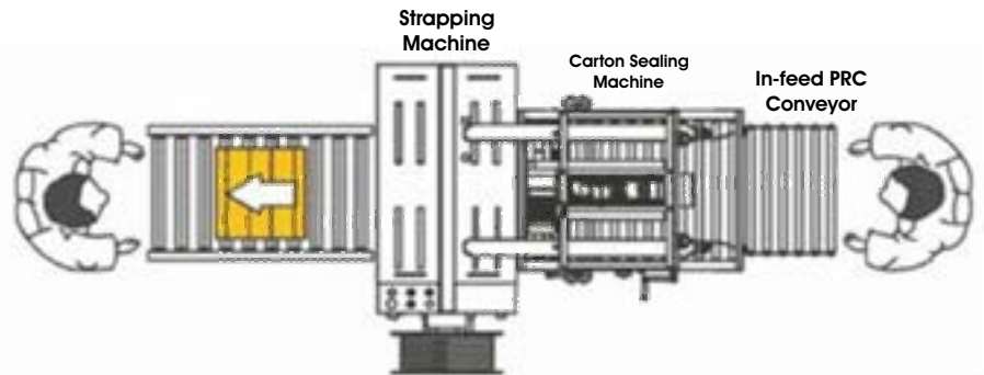
Automatic Flaps Folding Sealing Strapping Machine Solution II
