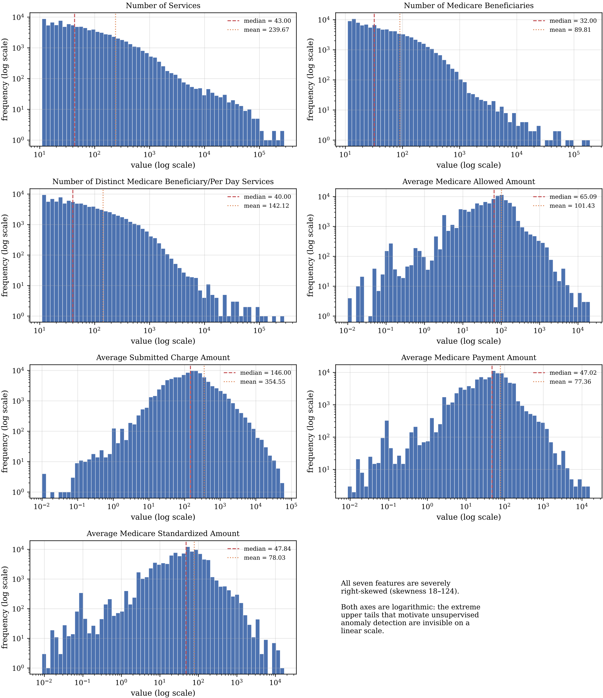
Figure 1. Distributions of the Seven Numerical Features (n = 100,000)
