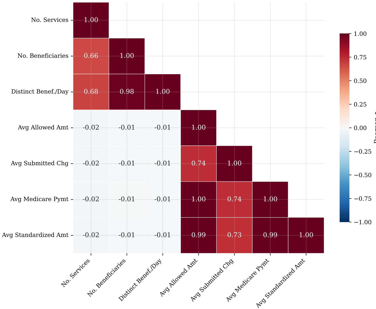
Figure 2. Pearson Correlation of Numerical Features
