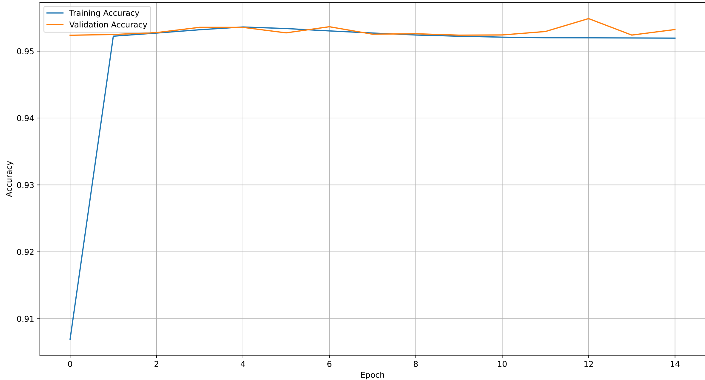
AUTOENCODER.pth -- Accuracy, Test Accuracy 0.948949011271062
