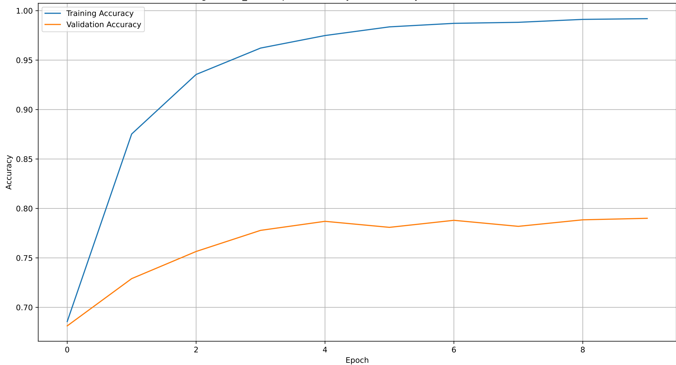
augmented_correct.pth -- Accuracy, Test Accuracy 0.7890466531440162
