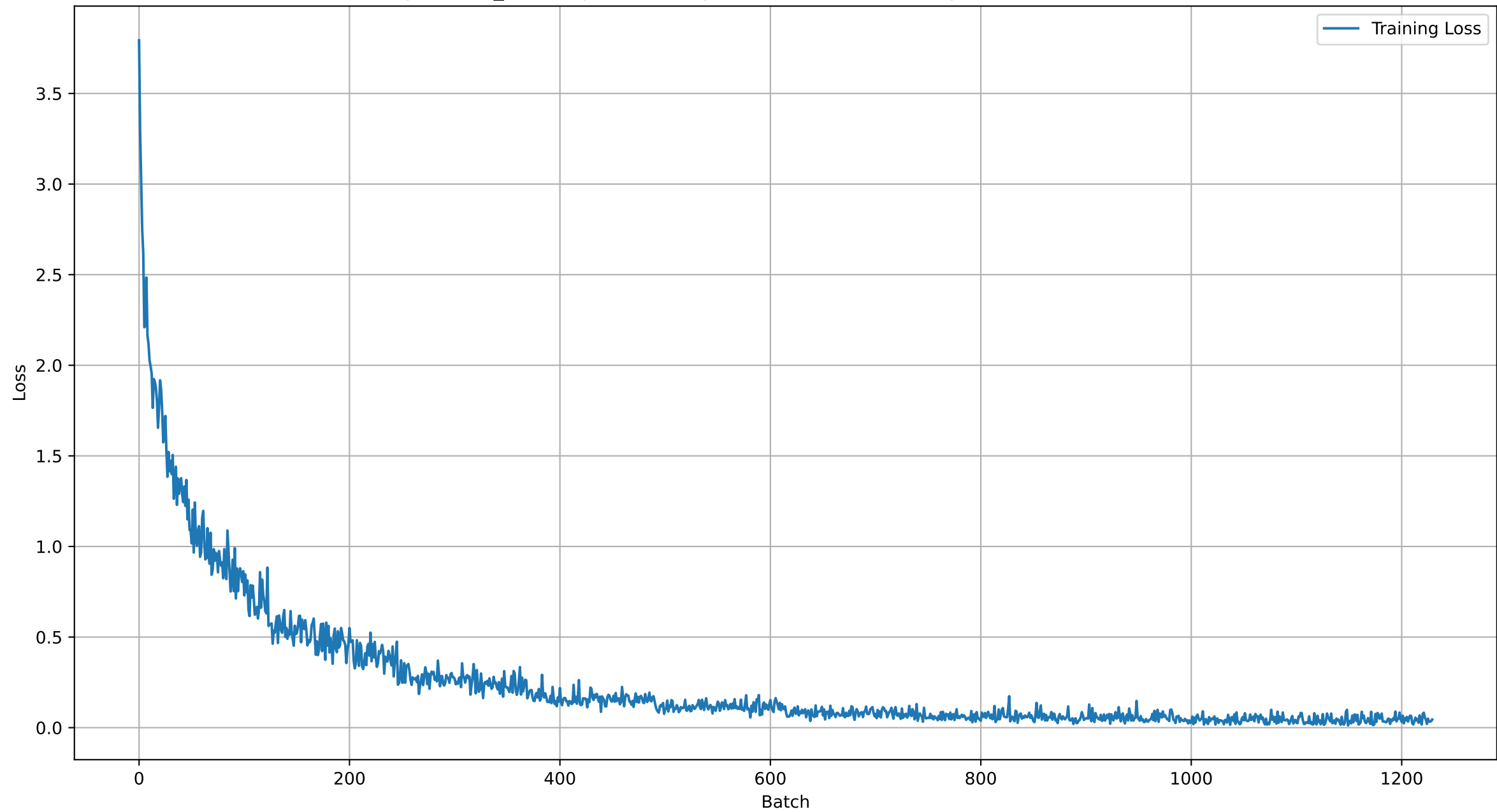
augmented_correct.pth -- Loss (per batch), Test Accuracy 0.7890466531440162
