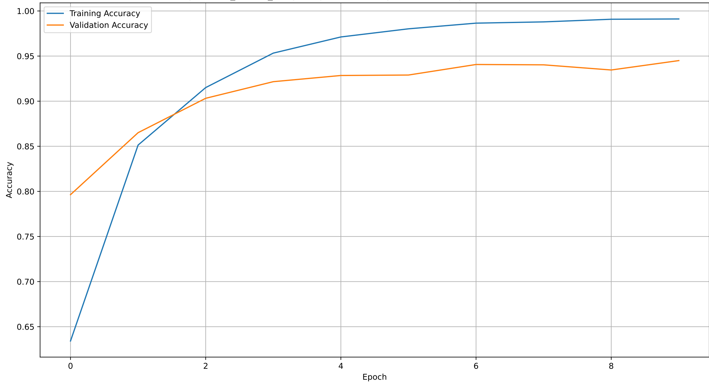
augmented_voxnet_leakyrelu.pth -- Accuracy, Test Accuracy 0.7910750507099391
