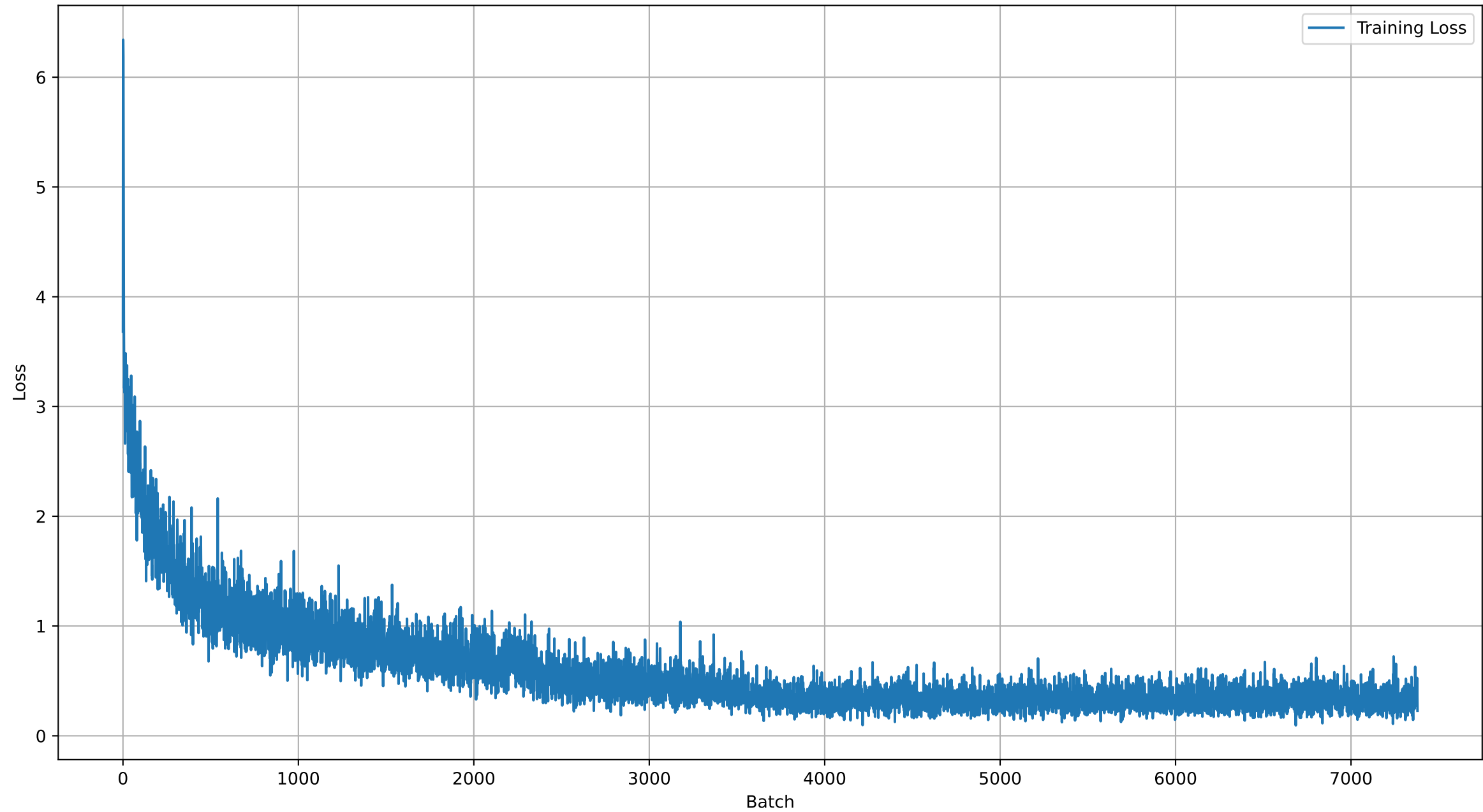
cont.pth -- Loss (per batch), Test Accuracy 0.8462474645030426
