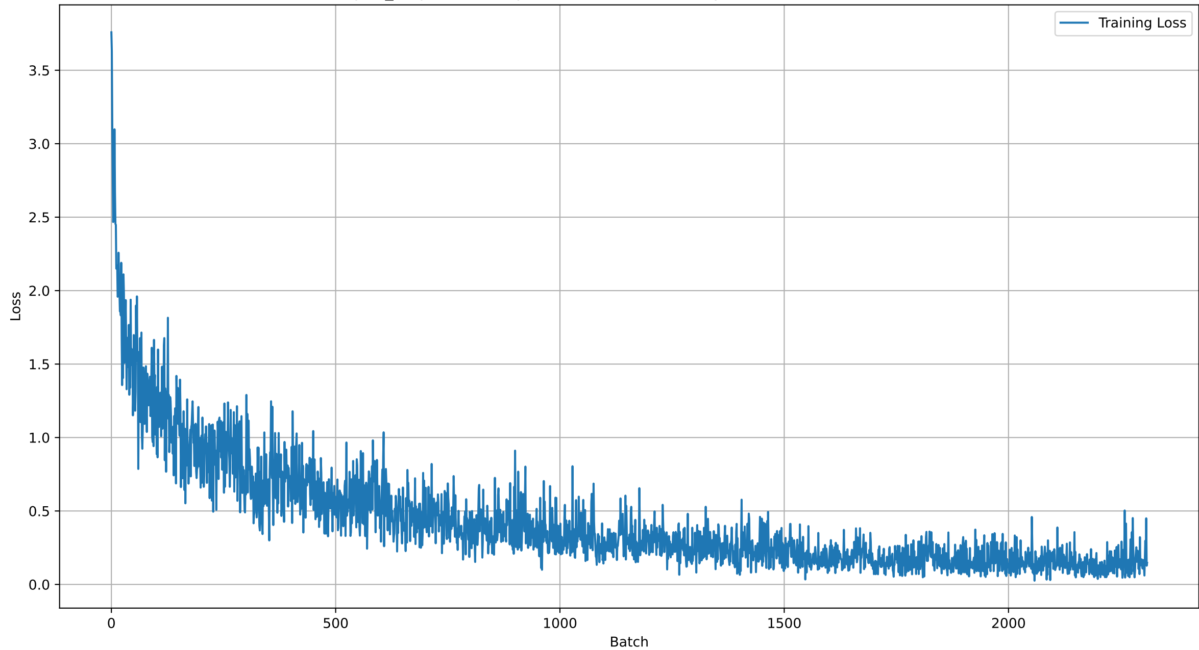
drop02_64.pth -- Loss (per batch), Test Accuracy {0.7844408427876823}
