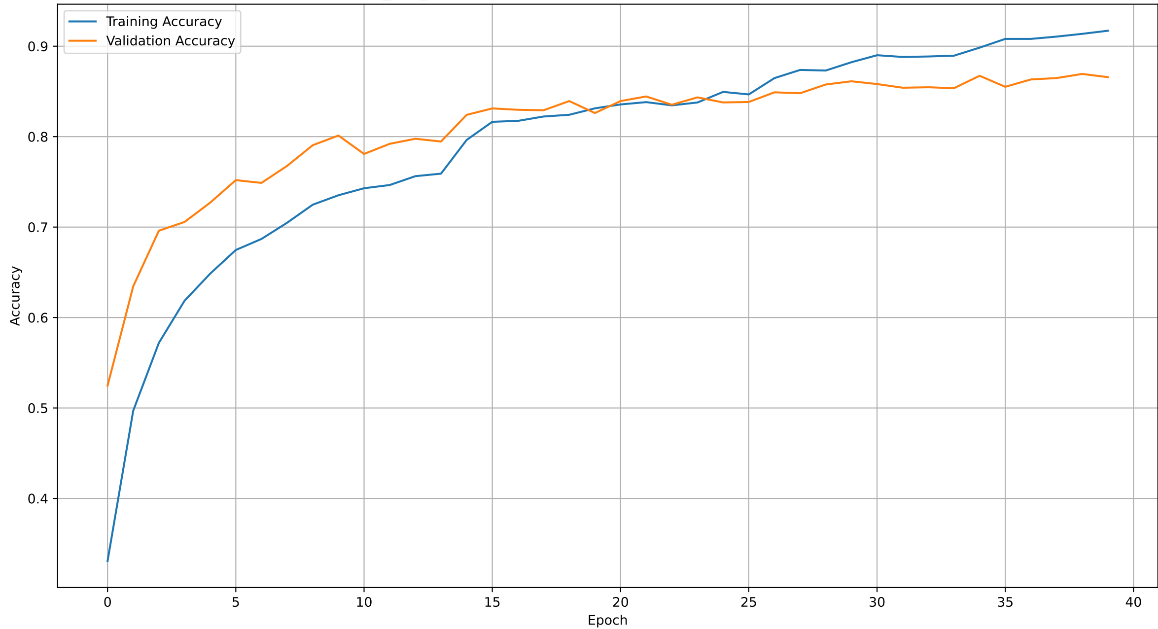
mixed_cnn_849.pth -- Accuracy, Test Accuracy 0.8494929006085192
