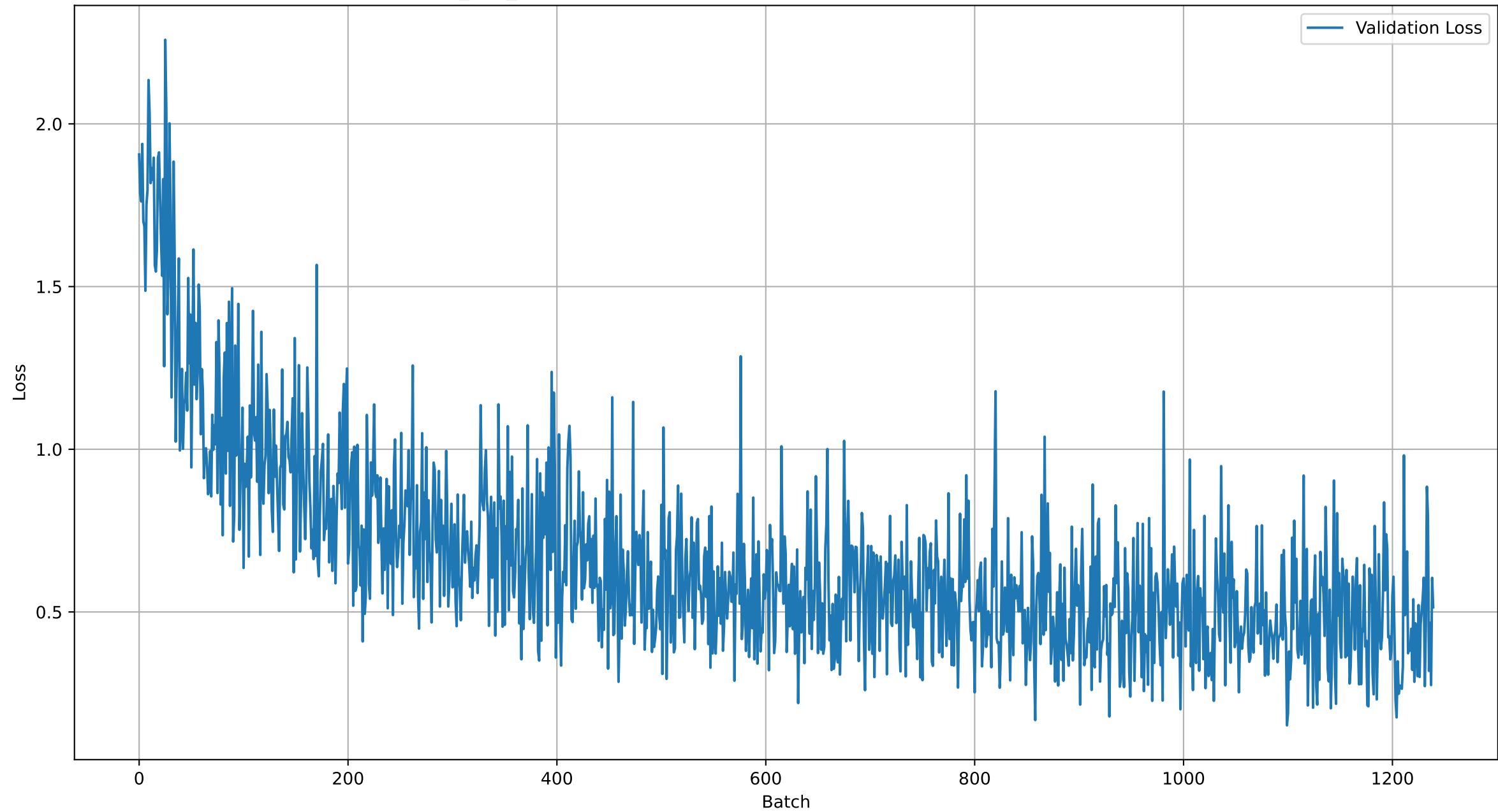
mixed_cnn_849.pth -- Loss (per batch), Test Accuracy 0.8494929006085192
