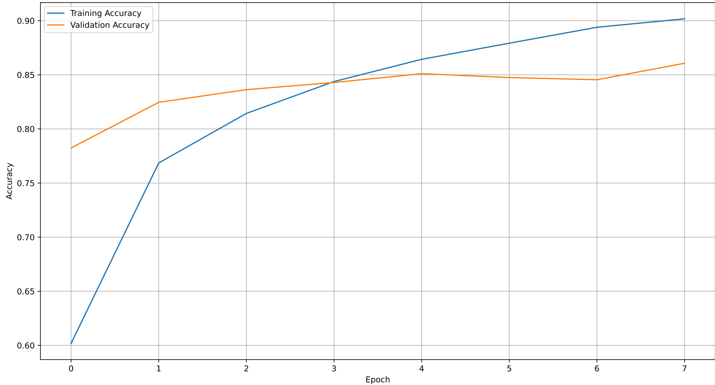
mixed_dimensional_fe.pth -- Accuracy, Test Accuracy 0.8316430020283976
