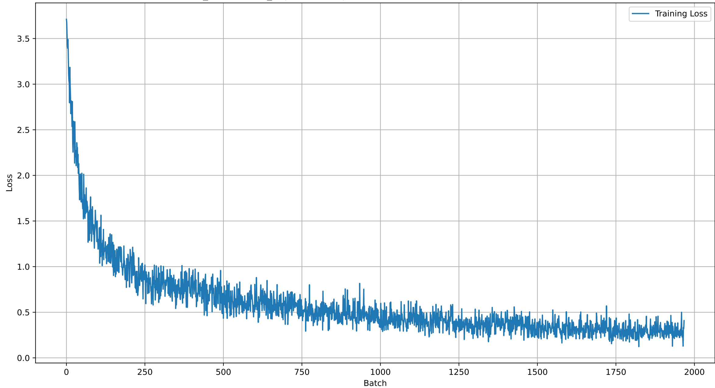
mixed_dimensional_fe.pth -- Loss (per batch), Test Accuracy 0.8316430020283976
