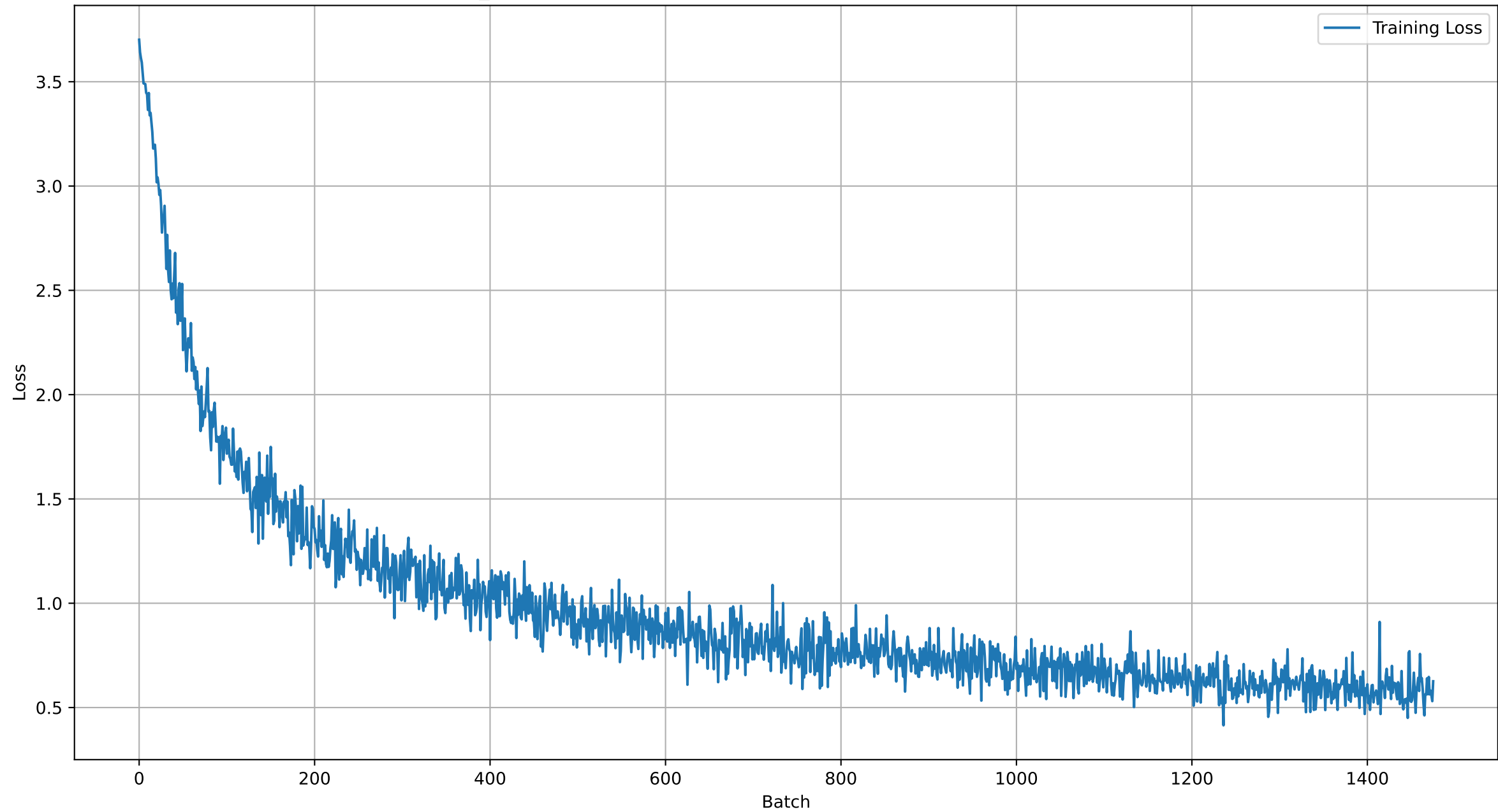
mixed_drop.pth -- Loss (per batch), Test Accuracy 0.7935091277890467
