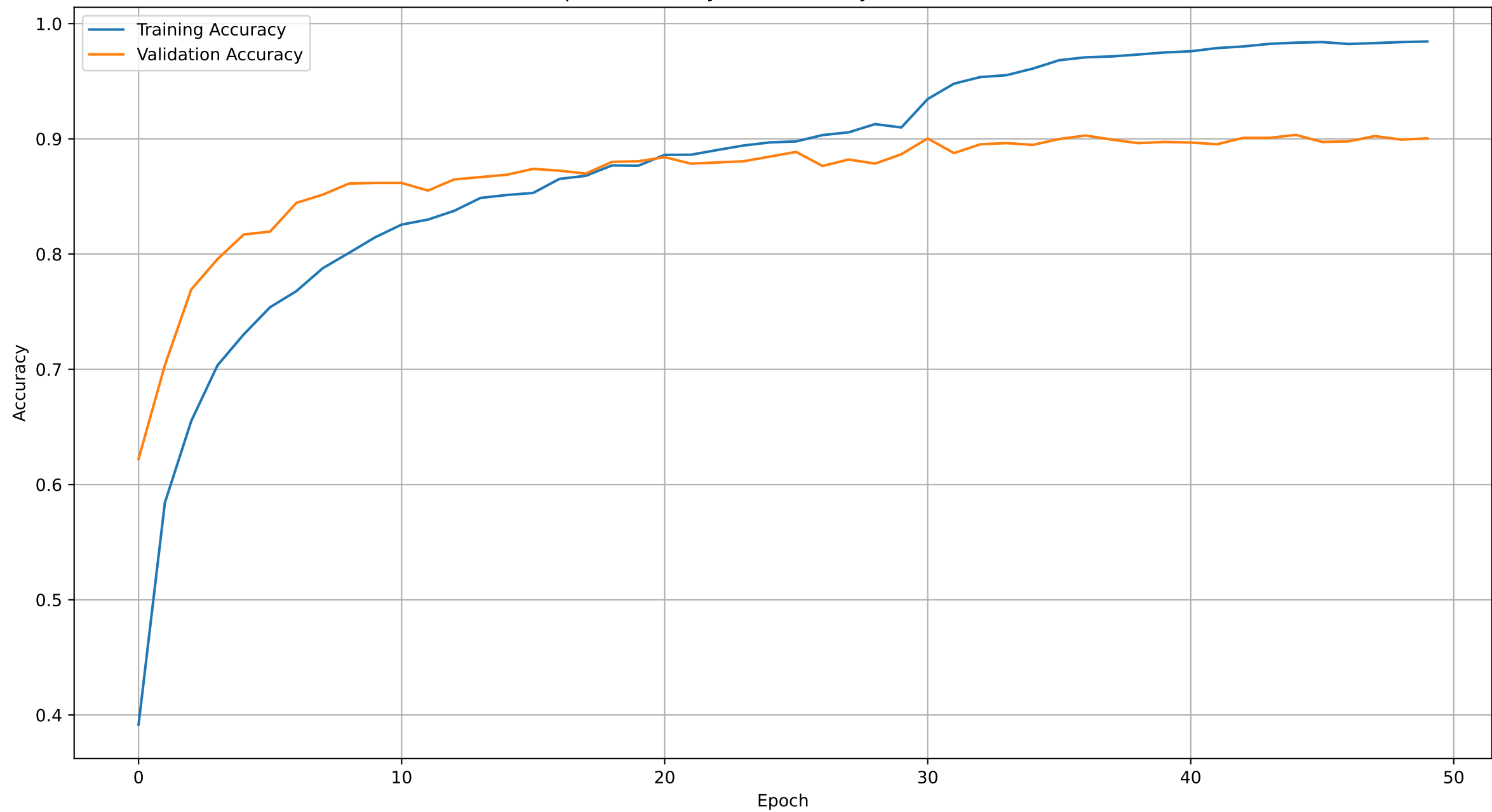
monster.pth -- Accuracy, Test Accuracy 0.867342799188641
