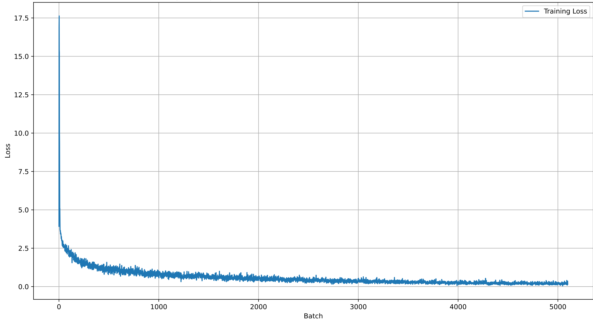
perm25.pth -- Loss (per batch), Test Accuracy 0.7330628803245436
