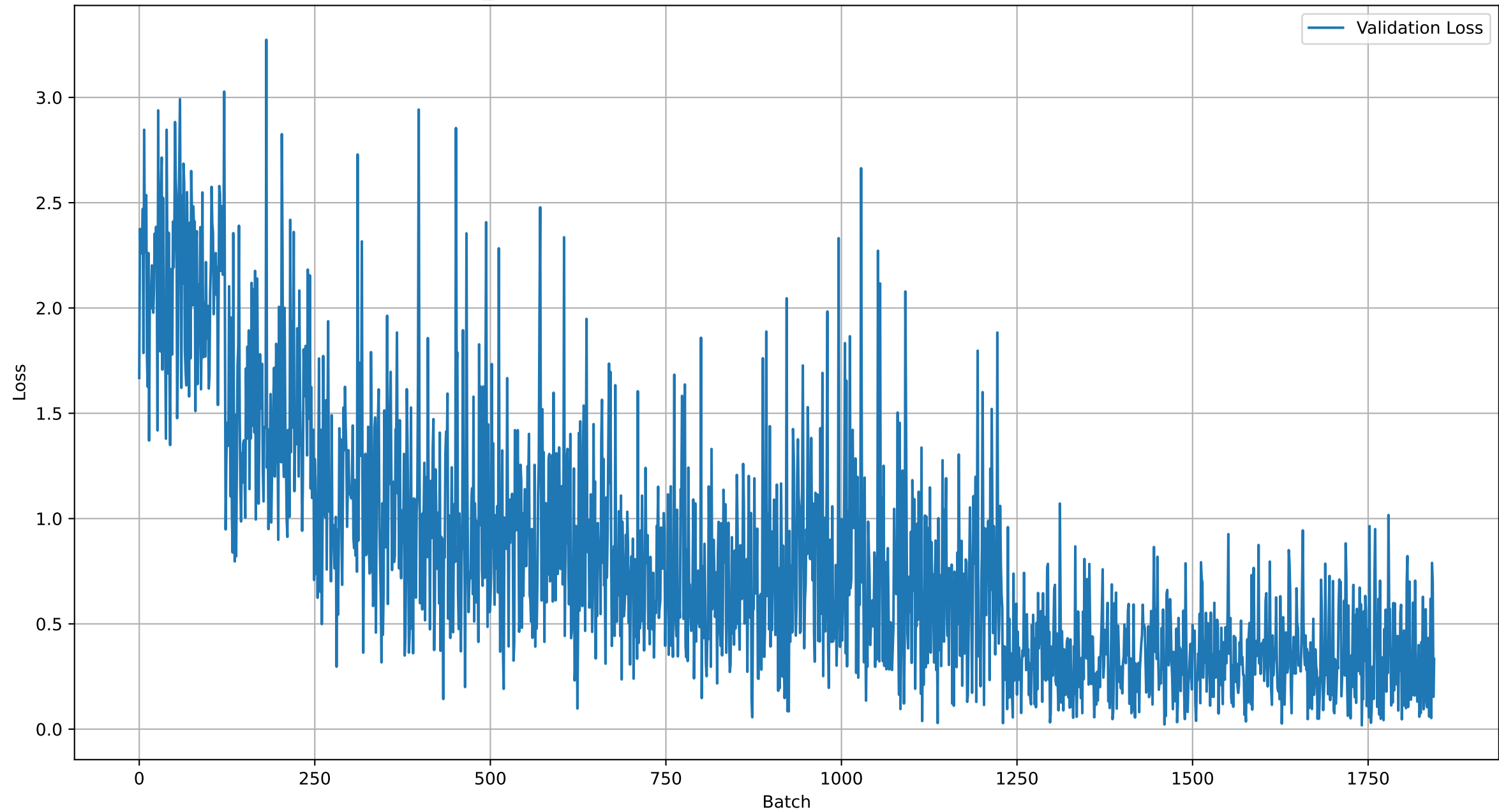
permute_noaug.pth -- Loss (per batch), Test Accuracy 0.7971602434077079
