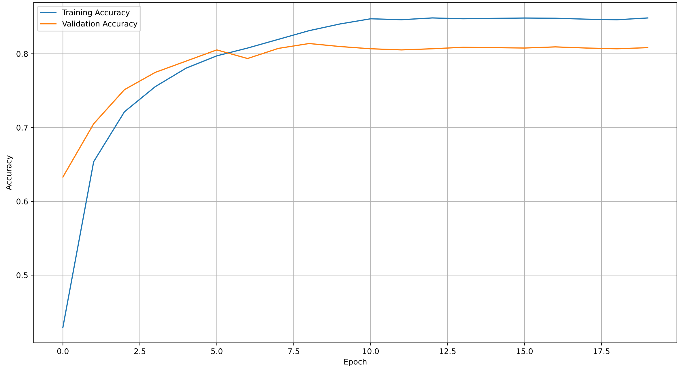
smalltwod.pth -- Accuracy, Test Accuracy 0.7894523326572008
