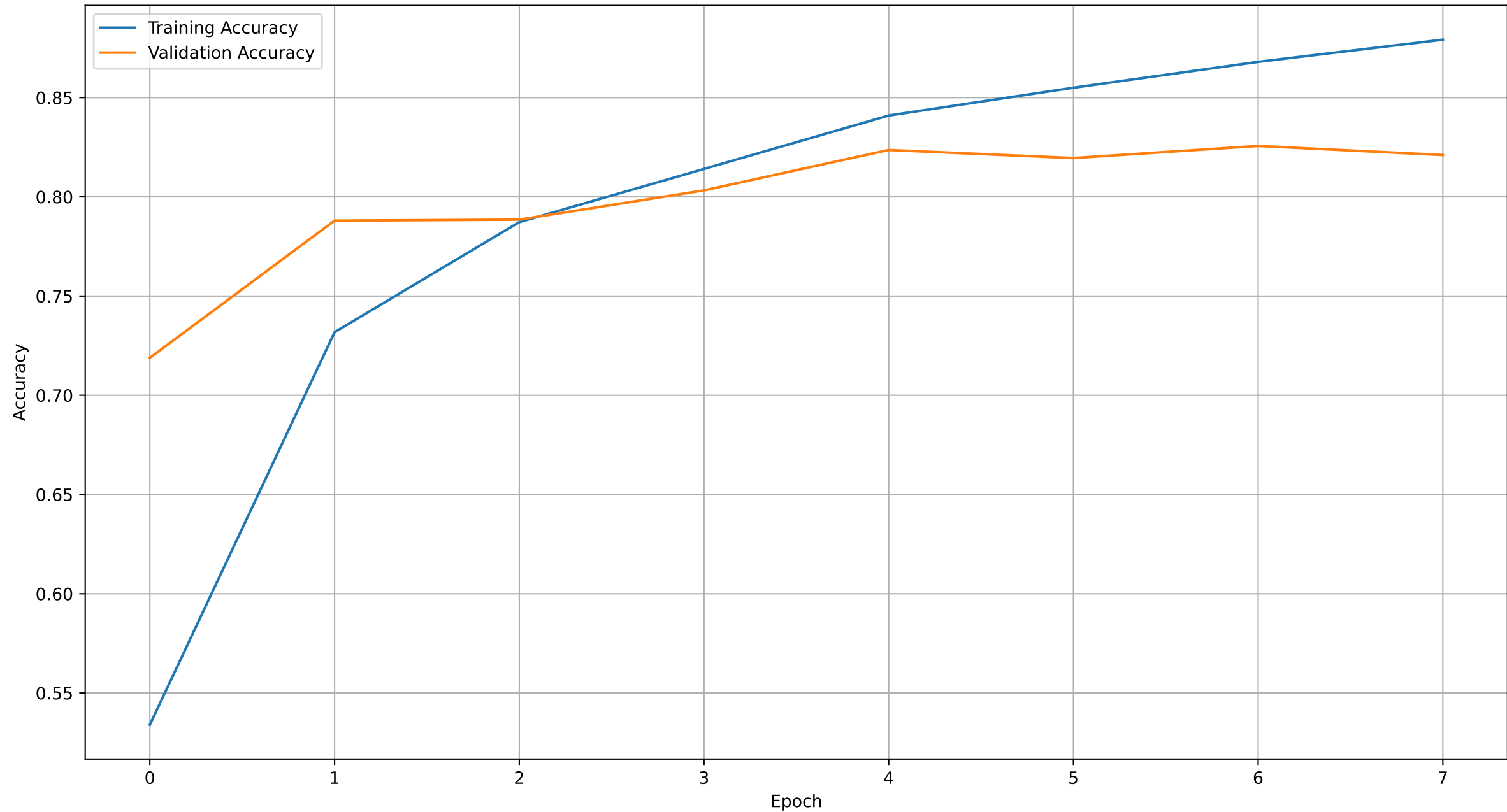
threelinear.pth -- Accuracy, Test Accuracy 0.8150101419878296
