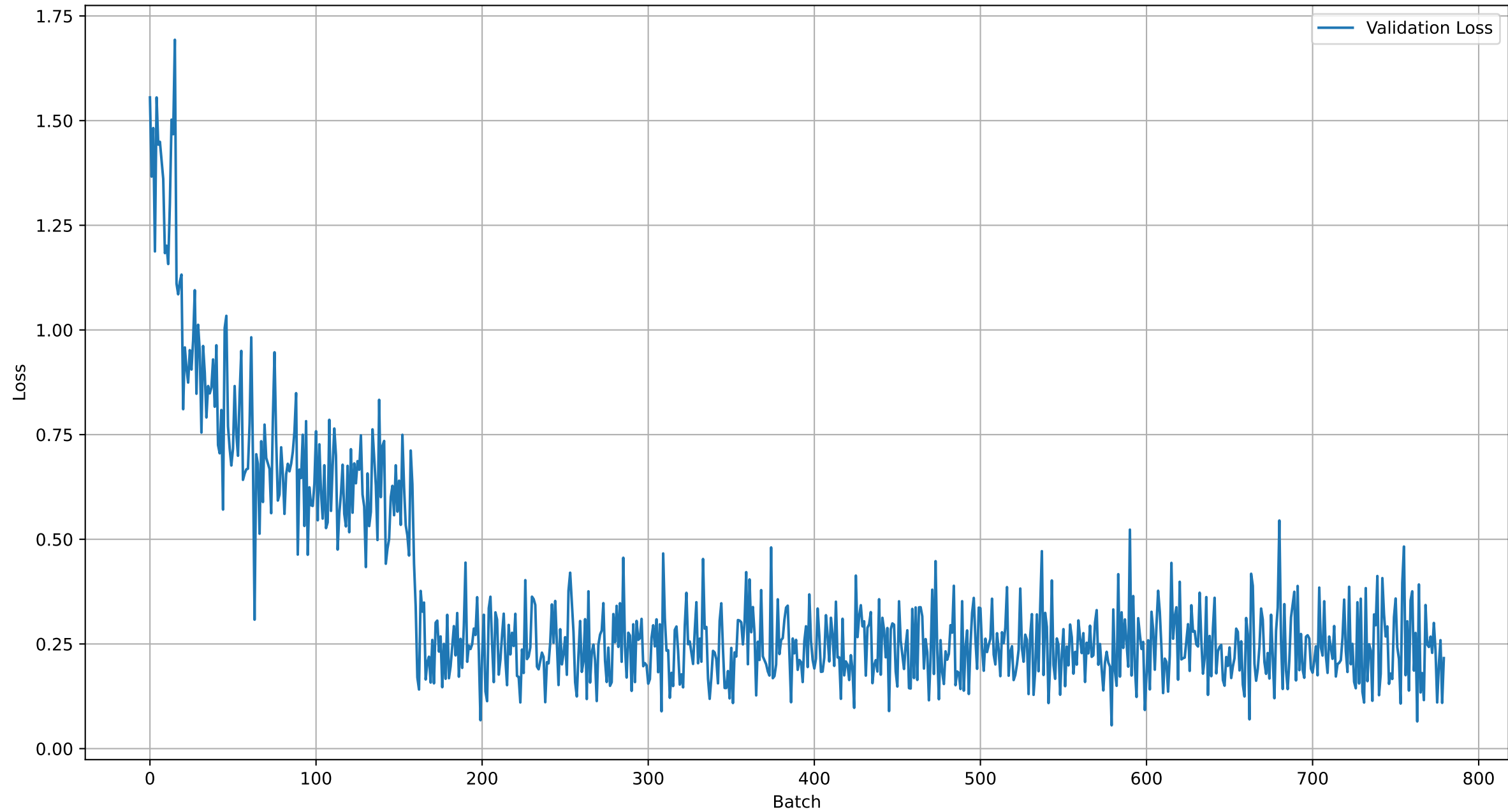
twopointfourmil.pth -- Loss (per batch), Test Accuracy 0.8105476673427991
