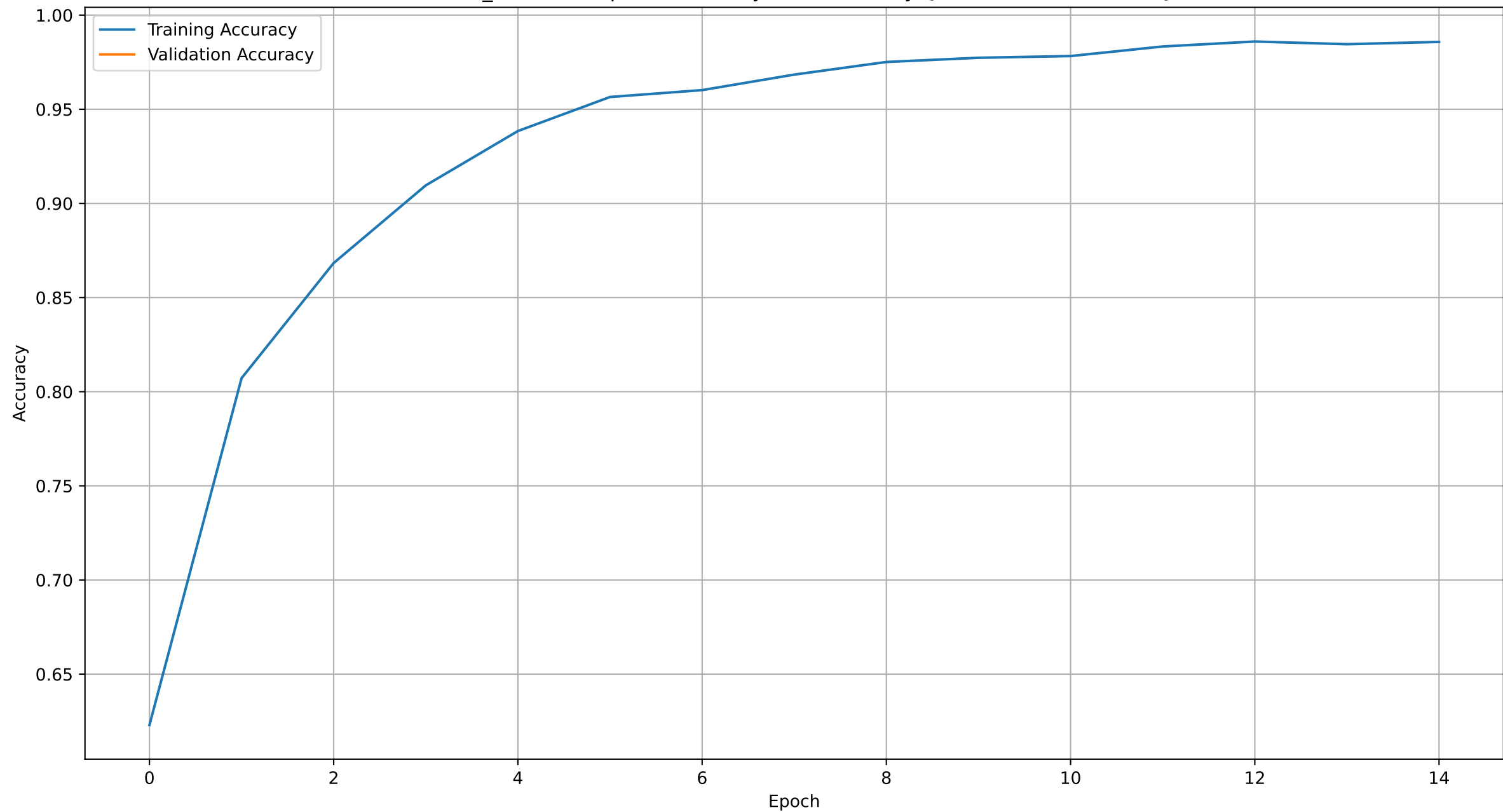
voxnet_batchnorm.pth -- Accuracy, Test Accuracy {0.7828200972447326}
