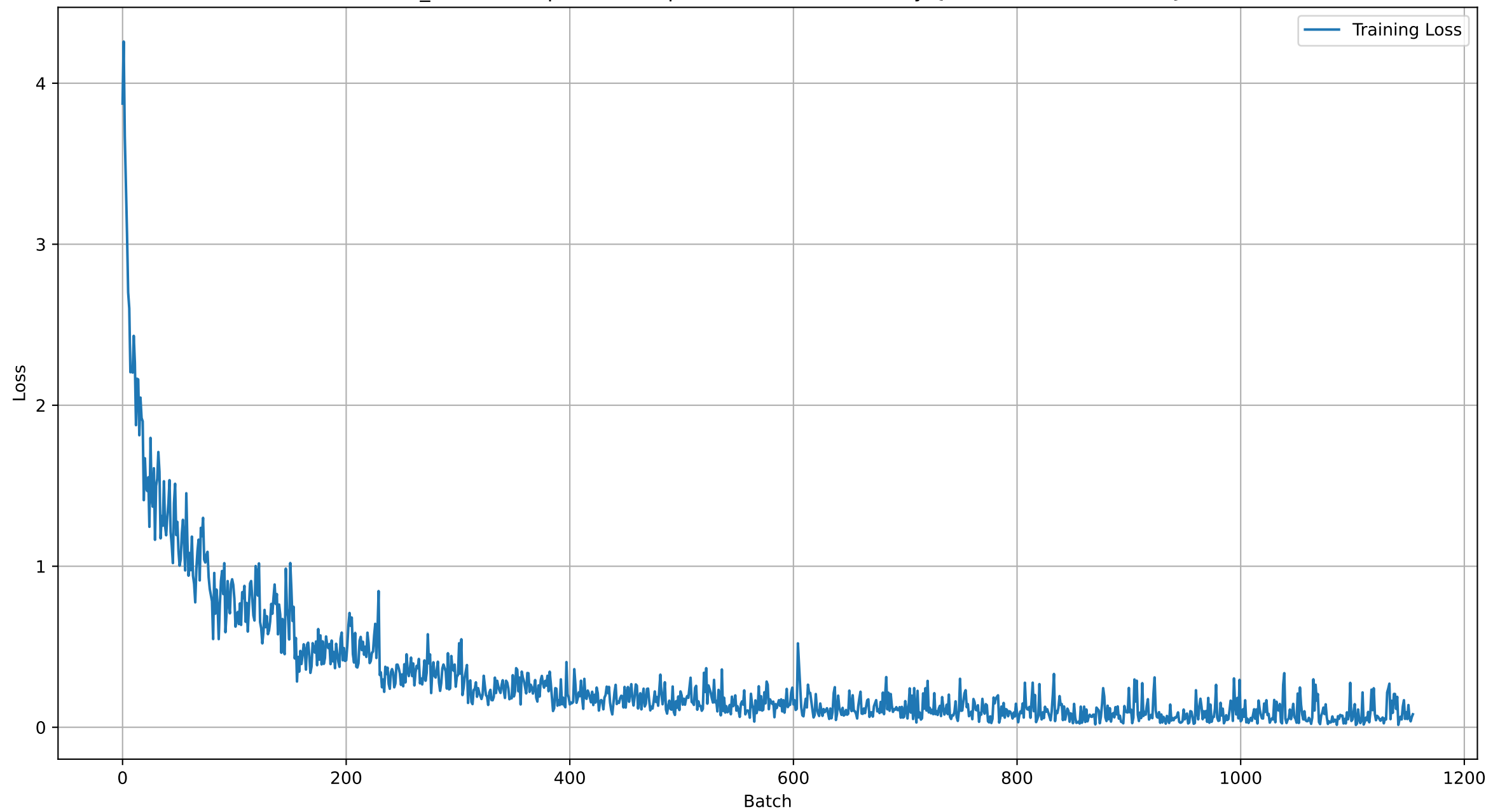
voxnet_batchnorm.pth -- Loss (per batch), Test Accuracy {0.7828200972447326}
