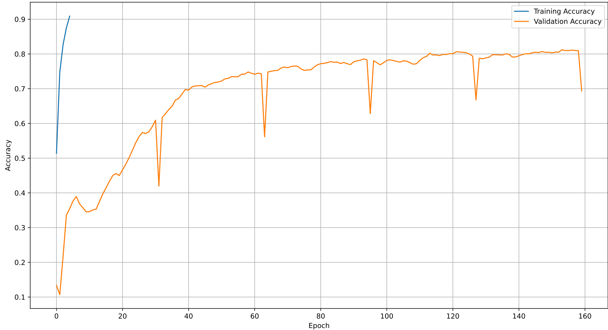
voxnet_batchnorm_relu_validation.pth -- Accuracy, Test Accuracy {0.7860615883306321}
