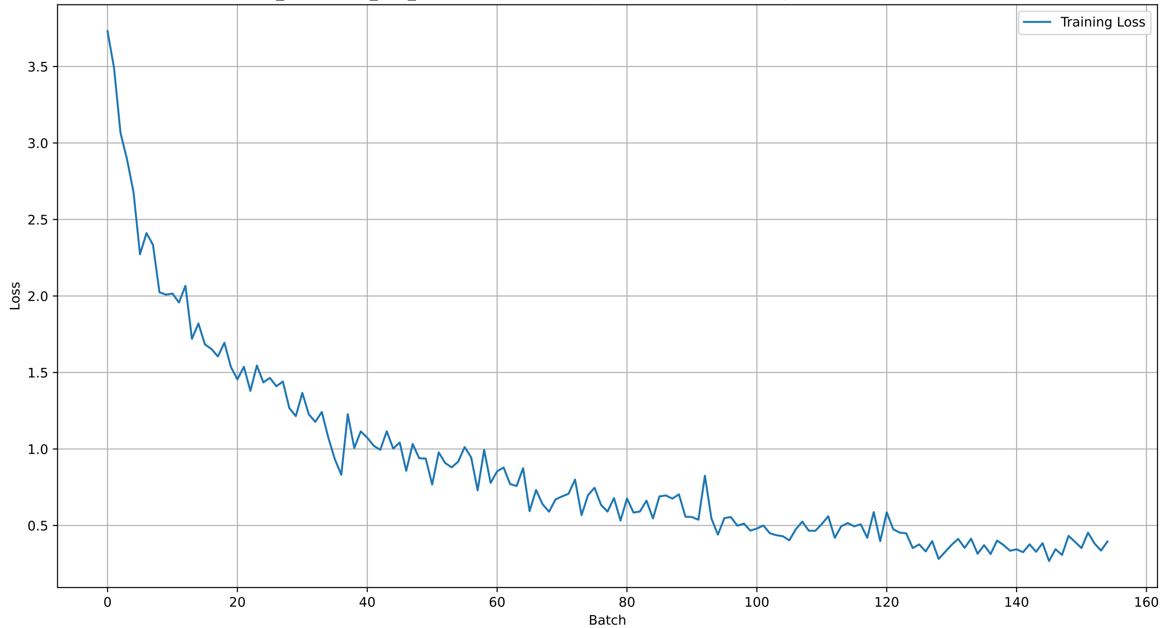
voxnet_batchnorm_relu_validation.pth -- Loss (per batch), Test Accuracy {0.7860615883306321}
