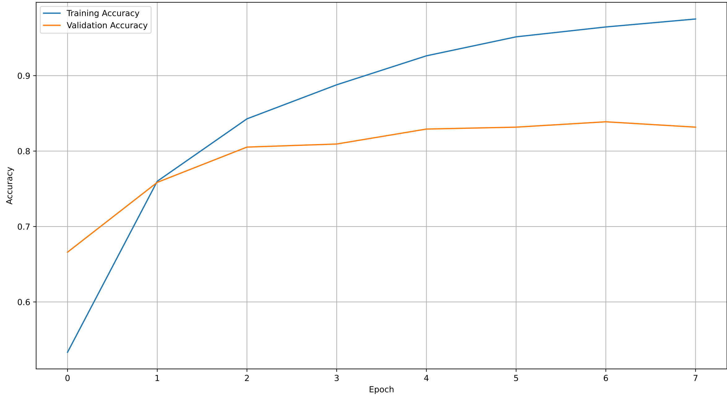
voxnet_leakyrelu.pth -- Accuracy, Test Accuracy 0.8081135902636917
