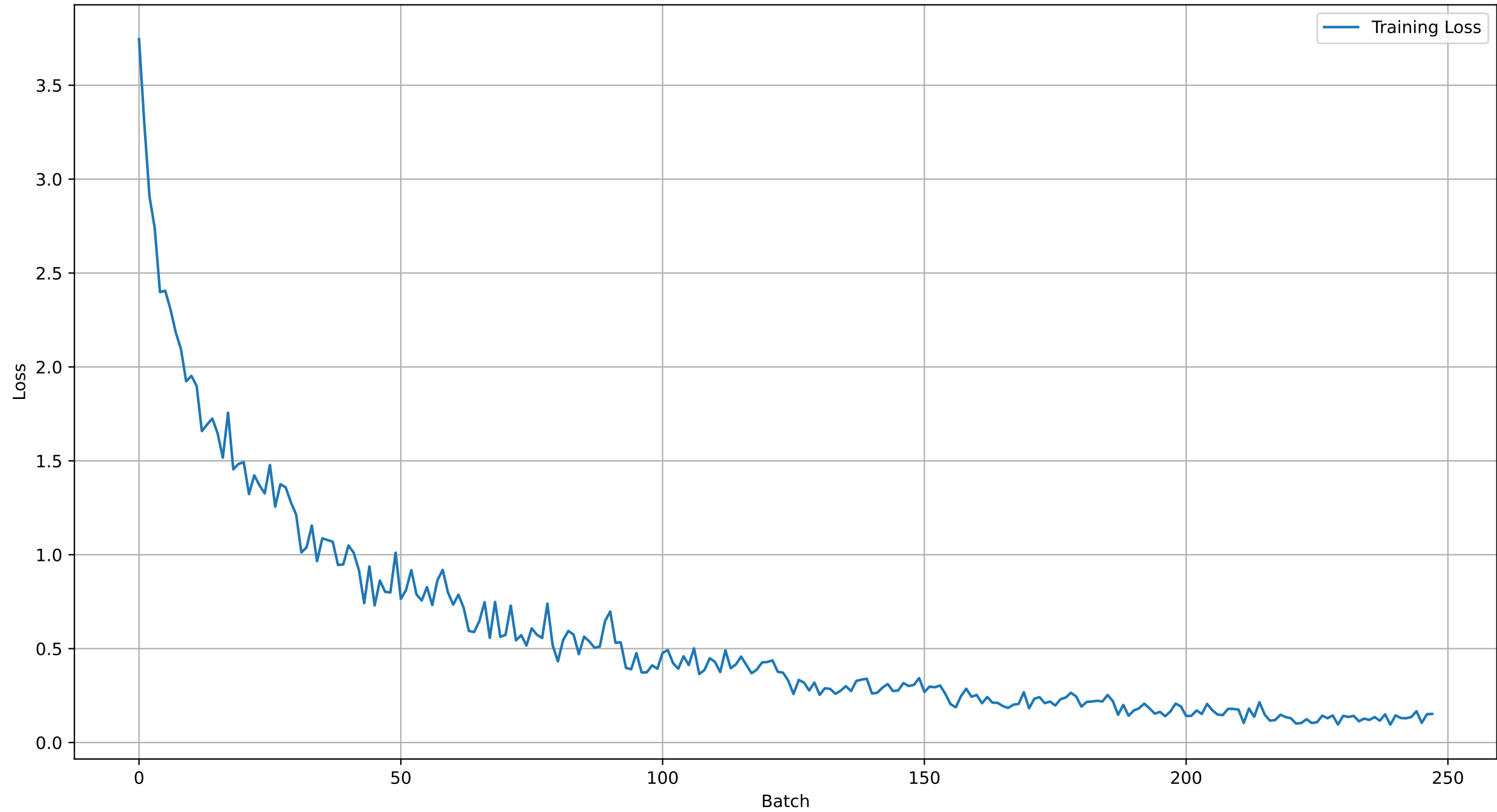
voxnet_leakyrelu.pth -- Loss (per batch), Test Accuracy 0.8081135902636917
