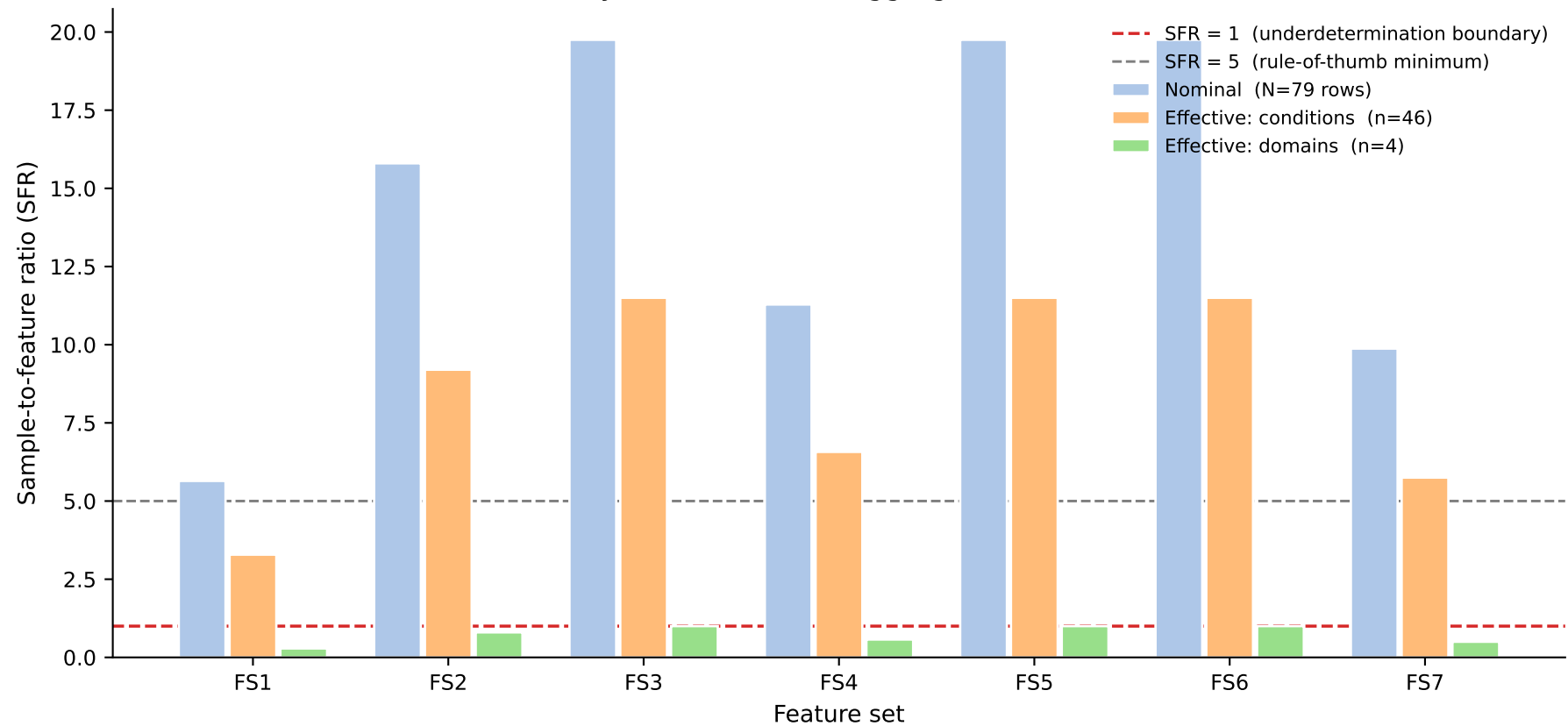
Nominal vs effective sample-to-feature ratio by feature set and aggregation level
