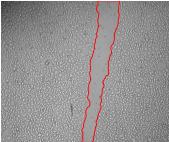
AI segmentation
